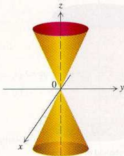
An elliptic double cone.
