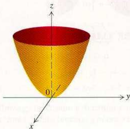
An elliptic paraboloid.
