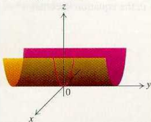
Two hyperbolic sheets.
