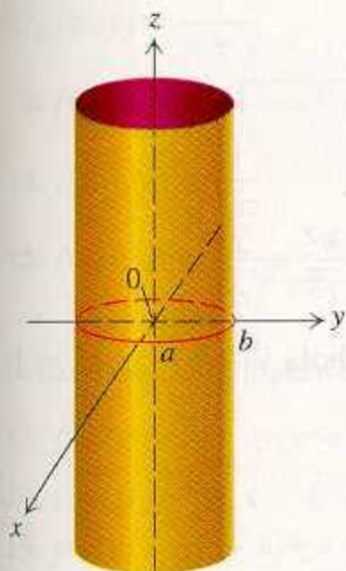
An elliptic cylinder
